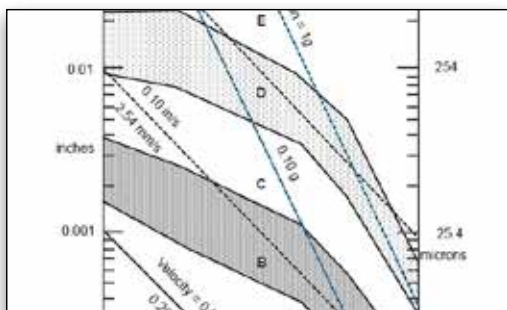
Dynamic ACI 351 charts for vibrating machine foundations
