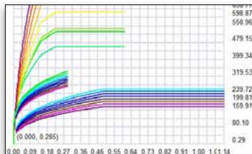
p-y curve generation for lateral analysis of drilled p
